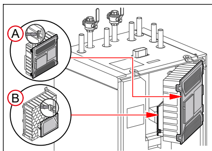
[A] XCU-THH-Klemmkasten
